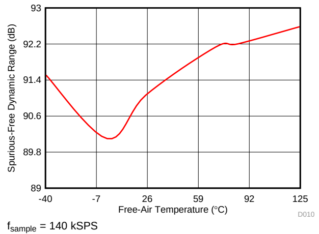
Figure 10. SFDR in Manual Mode with Temperature
