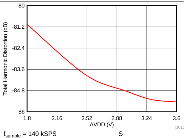
Figure 11. THD in Manual Mode with AVDD
