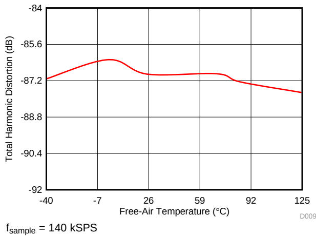
Figure 9. THD in Manual Mode with Temperature
