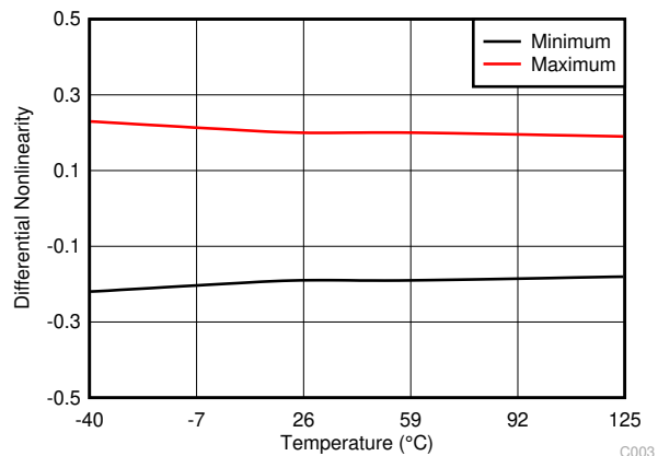
Figure 7-3. Typical DNL
