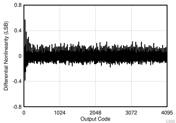
Figure 7-3. Typical DNL
