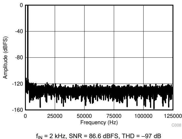
Figure 8-2. Test Results for the Single-Supply DAQ Circuit
