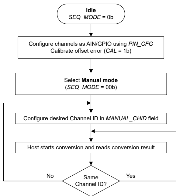
Figure 7-12. Device Operation in Manual Mode
