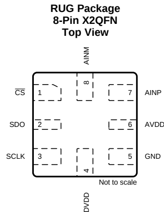
Pin Functions
