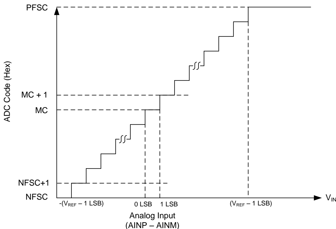
Figure 35. Ideal Transfer Characteristics
