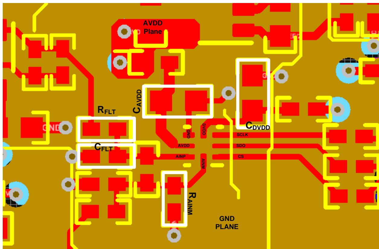
Figure 51. Example Layout
