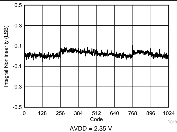
Figure 16. Typical INL
