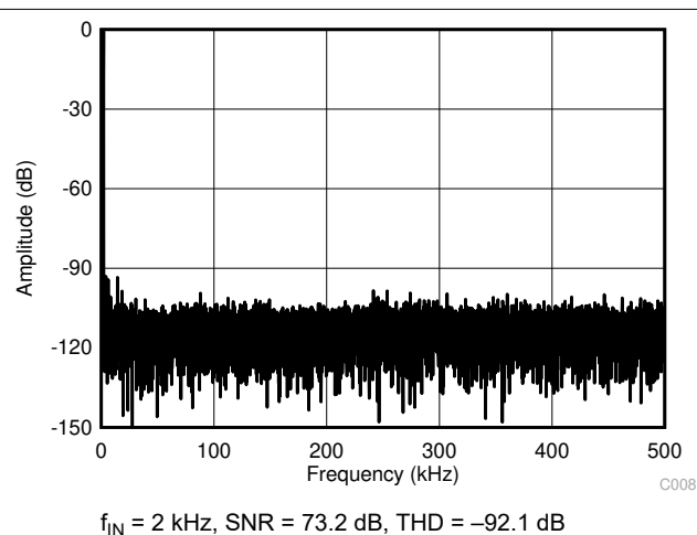
Figure 7-4. Typical FFT
