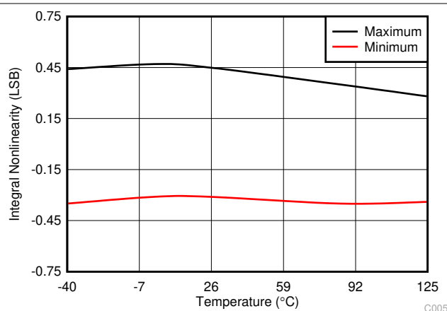
Figure 7-6. Typical INL
