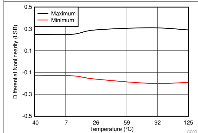
Figure 7-5. Typical DNL
