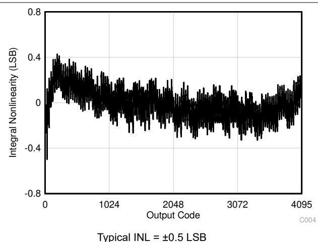
Figure 7-6. Typical INL
