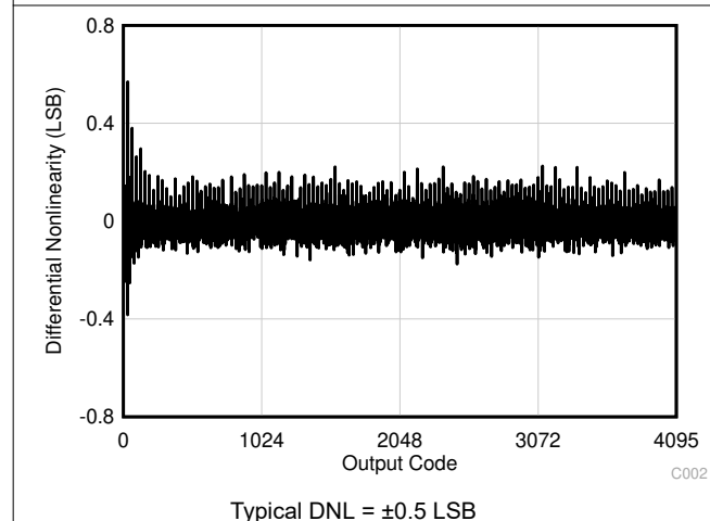
Figure 7-5. Typical DNL
