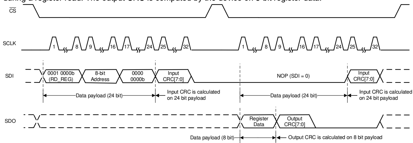
Figure 7-12. Register Read With CRC
