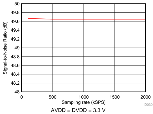
Figure 26. SNR vs Sampling Rate
