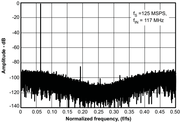
Figure 38. Spectrum with SNRBoost enabled
