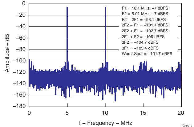
Figure 25. Intermodulation Distortion
