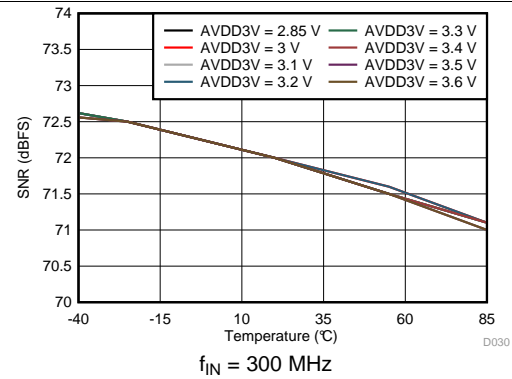
Figure 32. Signal-to-Noise Ratio vs AVDD3V Supply and Temperature
