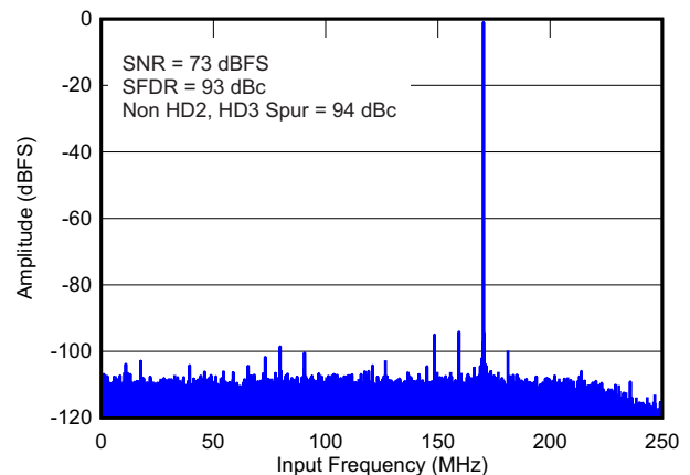
Spectrum at 170-MHz IF
