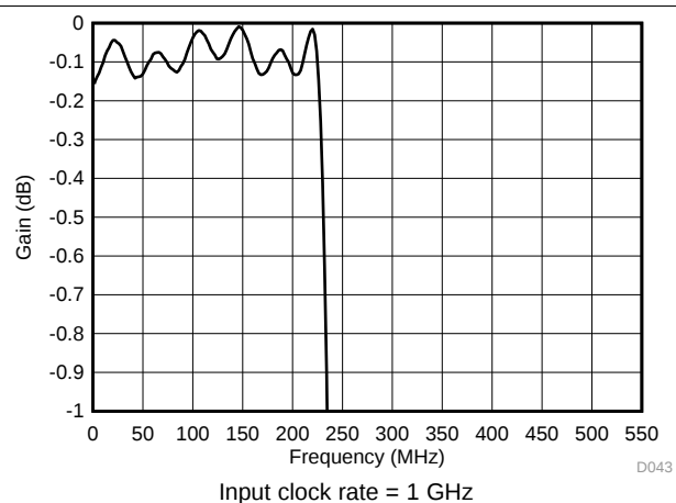
Figure 51. Decimation Filter Pass-Band Ripple vs Frequency
