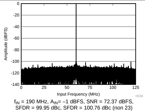
Figure 37. FFT for 190-MHz Input Signal
