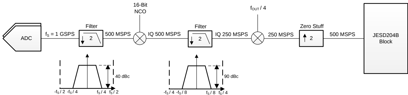
Figure 60. Operating Mode 7
