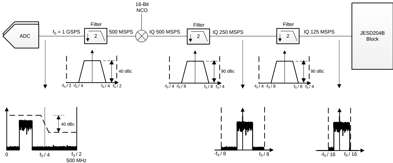
Figure 59. Operating Mode 6
