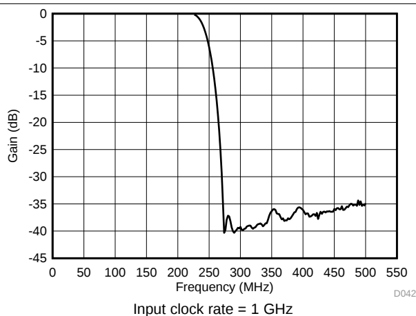
Figure 50. Decimation Filter Response vs Frequency
