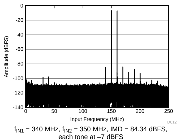
Figure 13. FFT for Two-Tone Input Signal
