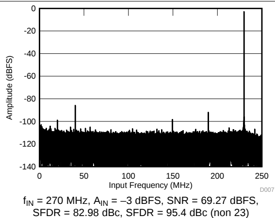
Figure 8. FFT for 270-MHz Input Signal
