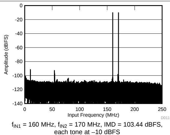
Figure 12. FFT for Two-Tone Input Signal
