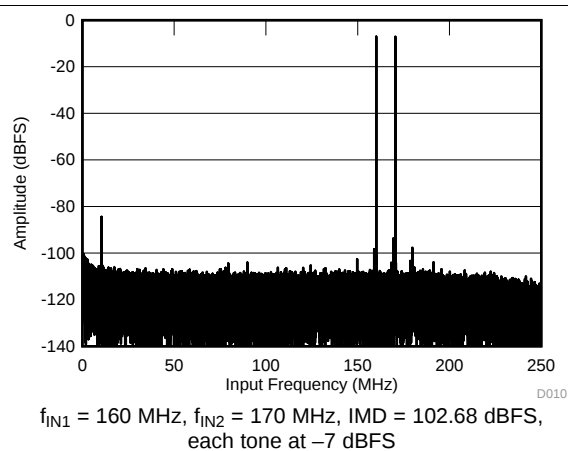
Figure 11. FFT for Two-Tone Input Signal
