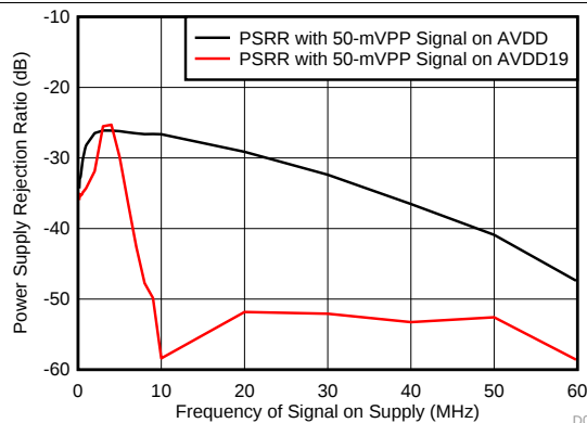
Figure 32. PSRR vs Power-Supply Noise Frequency
