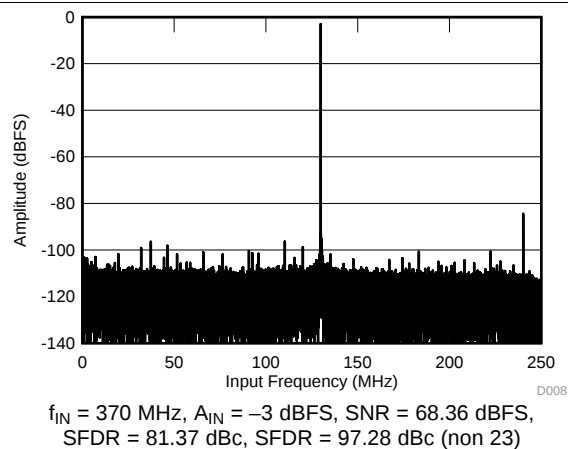
Figure 9. FFT for 370-MHz Input Signal
