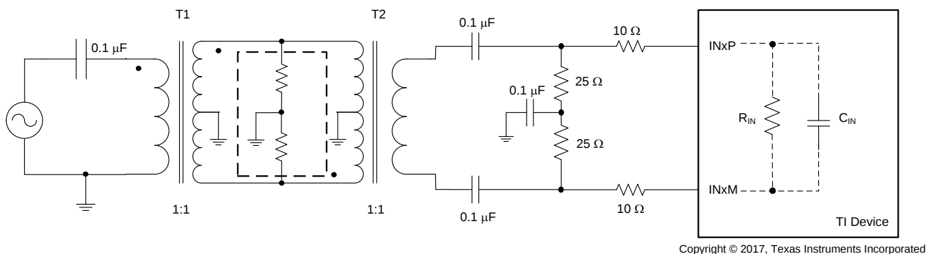
Figure 46. Analog Input Driving Circuit
