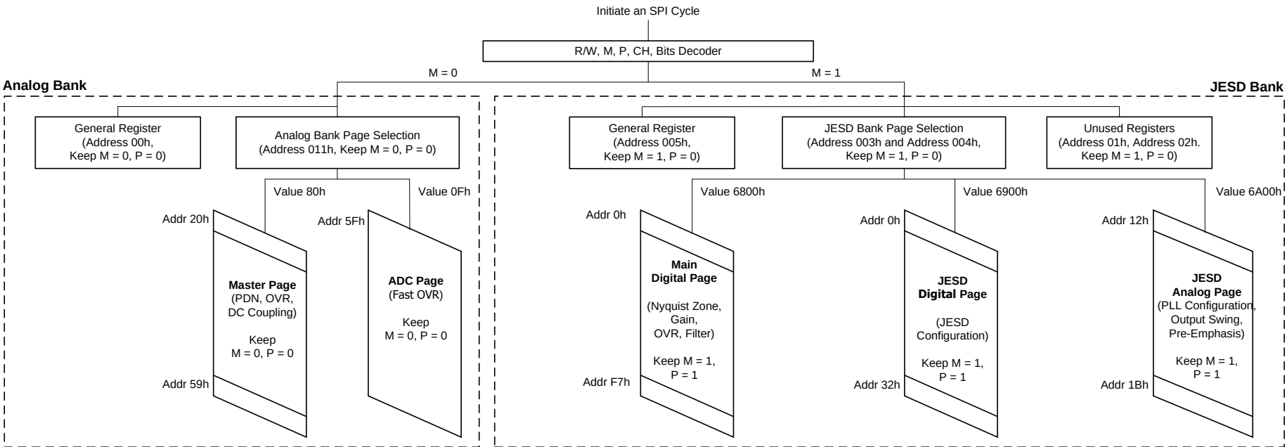
Figure 81. Serial Interface Registers
