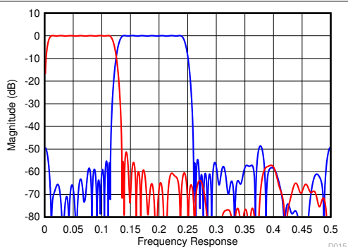
Figure 8-6. Decimate-by-4 Filter Response
