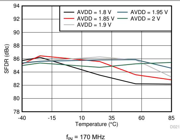
Figure 7-24. Spurious-Free Dynamic Range vs AVDD Supply and Temperature
