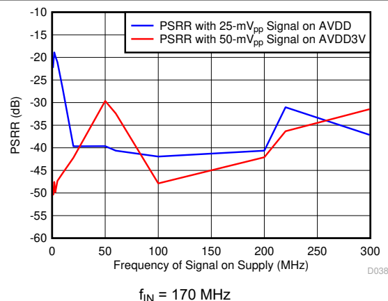
Figure 7-44. Power-Supply Rejection Ratio vs Test Signal Frequency
