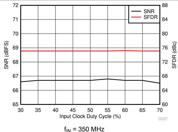
Figure 7-43. Performance vs Input Clock Duty Cycle
