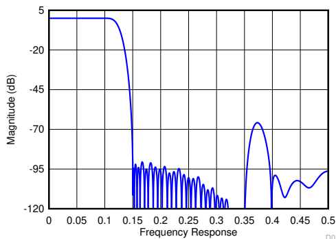
Figure 8-8. Decimate-by-4 IQ Output Filter Response
