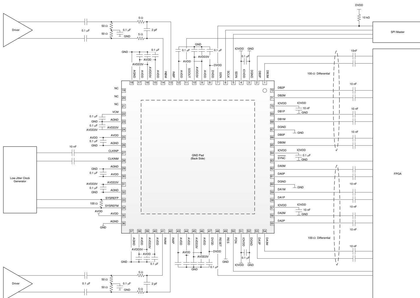
Figure 9-14. AC-Coupled Receiver
