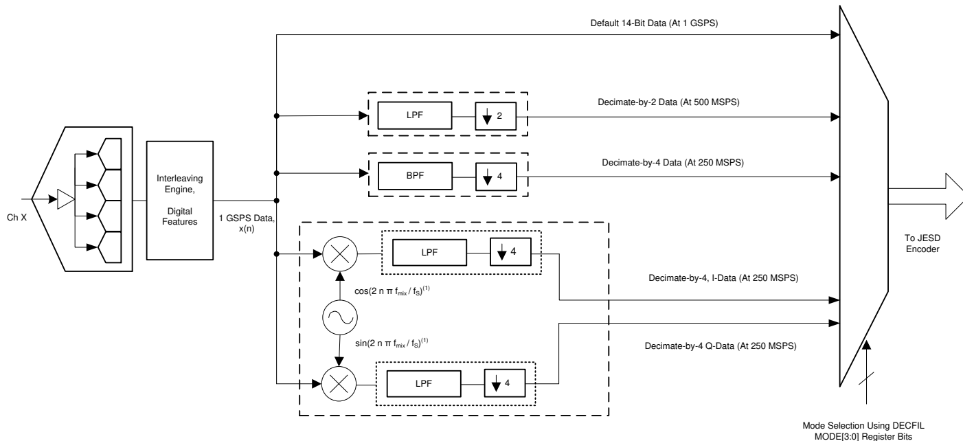
Figure 8-3. DDC Block
