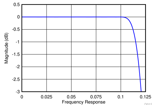
Figure 8-9. Decimate-by-4 IQ Output Filter Response (Zoomed)
