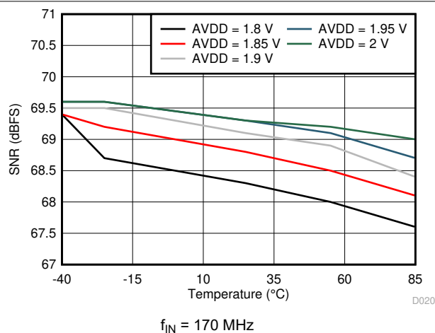
Figure 7-23. Signal-to-Noise Ratio vs AVDD Supply and Temperature
