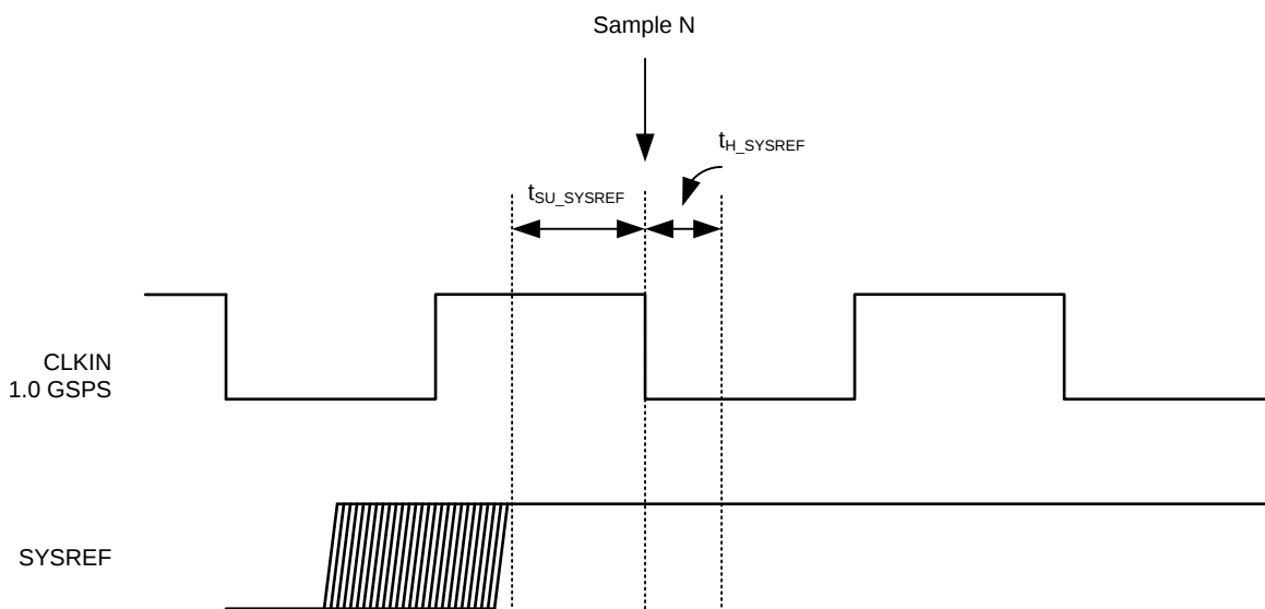
Figure 1. SYSREF Timing
