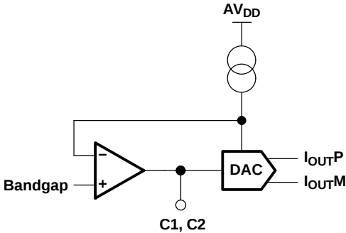
Figure 36. Decoupling Pin
