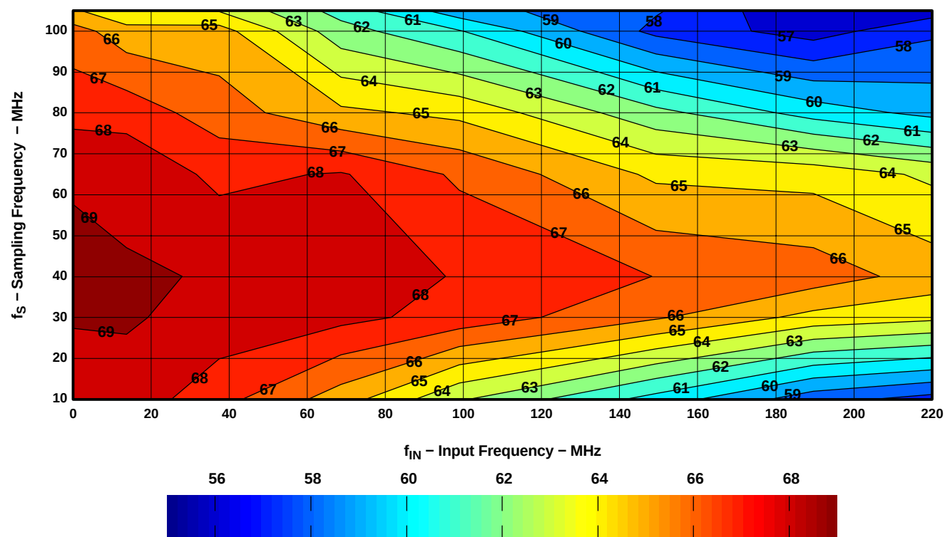
Figure 14. SNR– dBFS
