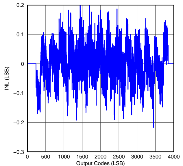
Figure 64. INTEGRAL NONLINEARITY
