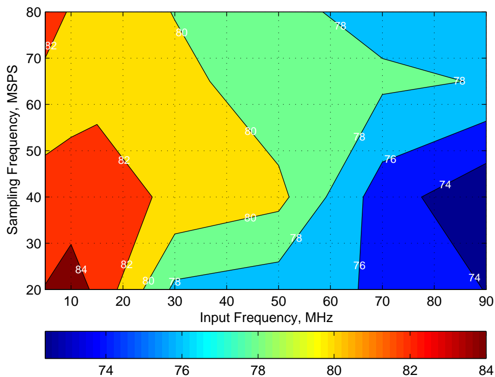
Figure 40. SPURIOUS-FREE DYNAMIC RANGE vs INPUT AND SAMPLING FREQUENCIES
