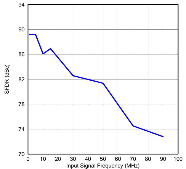
Figure 62. SPURIOUS-FREE DYNAMIC RANGE vs INPUT SIGNAL FREQUENCY
