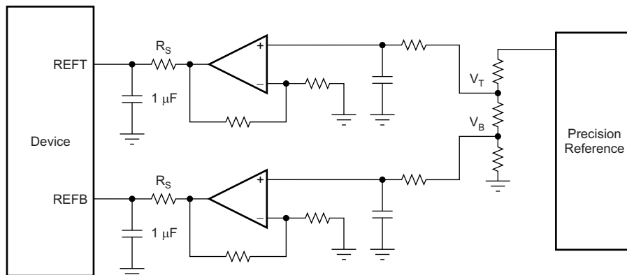
Figure 92. Driving Reference Inputs in External Reference Mode
