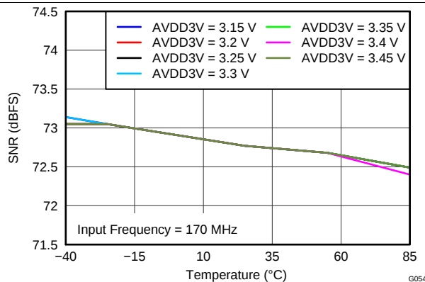
Figure 53. Signal-to-Noise Ratio vs AVDD Supply and Temperature (170 MHz)
