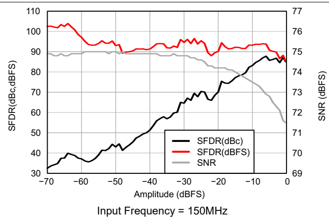
Figure 6-17. Performance vs Input Amplitude
