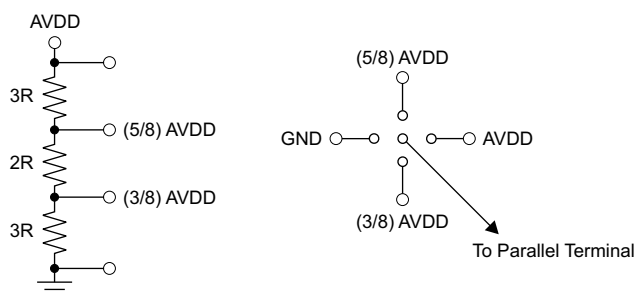
Figure 7-8. Simple Scheme To Configure The Parallel Terminals
