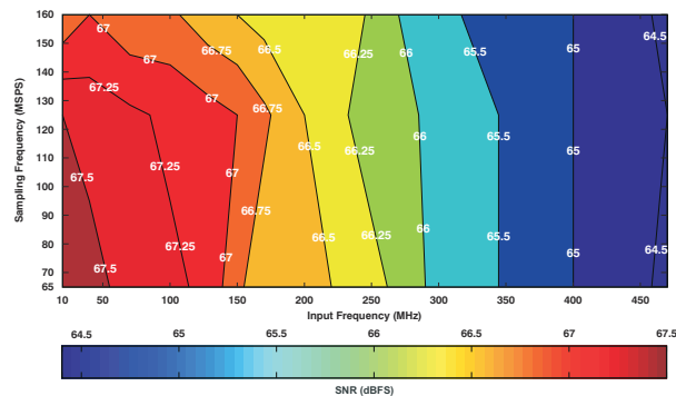
Figure 6-36. Signal-To-Noise Ratio (6dB Gain)
