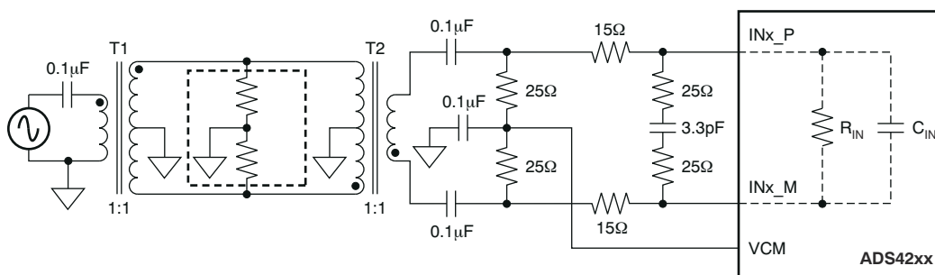
Figure 8-7. Drive Circuit With Low Bandwidth (For Low Input Frequencies Less Than 150MHz)
