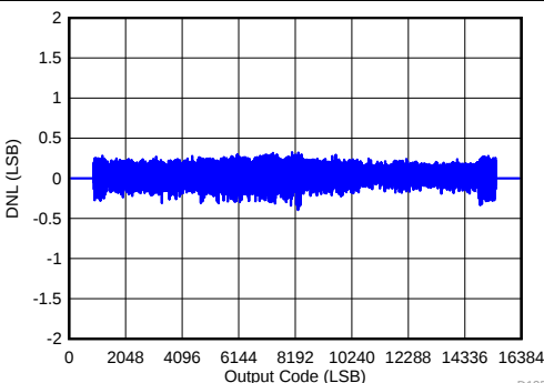
Figure 146. Differential Nonlinearity at 3-MSPS Sampling Speed
