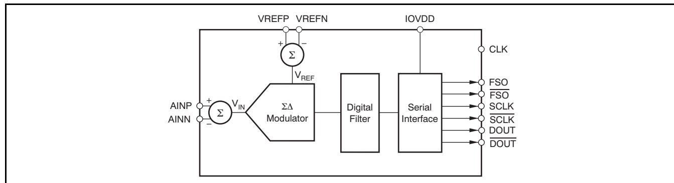
Figure 38. Conceptual Block Diagram
