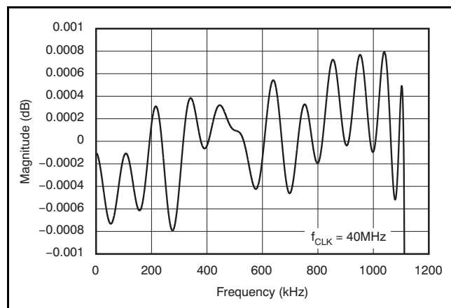
Figure 49. Passband Ripple
