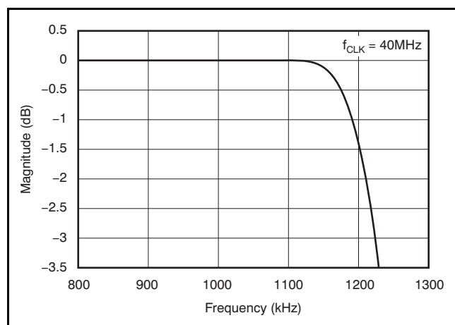
Figure 50. Passband Transition
