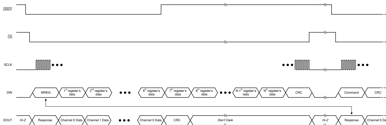
Figure 8-25. Writing Registers
