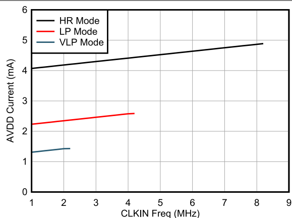
Figure 6-26. AVDD Current vs CLKIN Frequency
