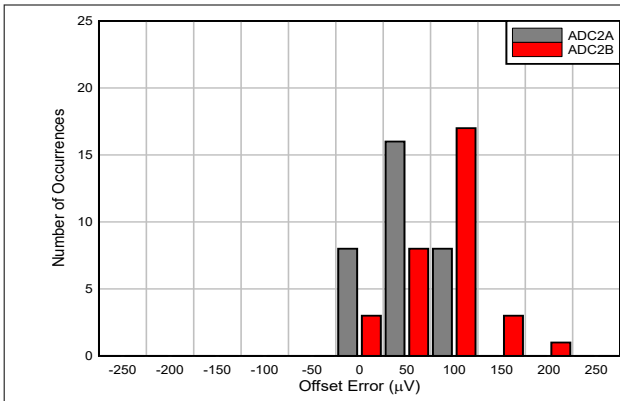
32 devices, gain = 1, input referred Figure 5-8. ADC2y Offset Error Histogram
