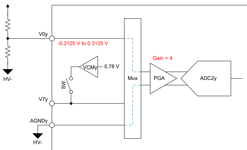
Figure 7-10. Single-Ended Input, Bipolar Voltage Measurement (Gain = 4)
