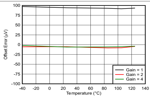
Input referred Figure 5-9. ADC2y Offset Error vs Temperature
