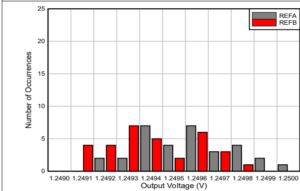
32 devices Figure 5-12. REFy Output Voltage Histogram
