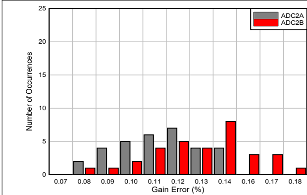
32 devices, gain = 1, including error of REFy Figure 5-10. ADC2y Gain Error Histogram
