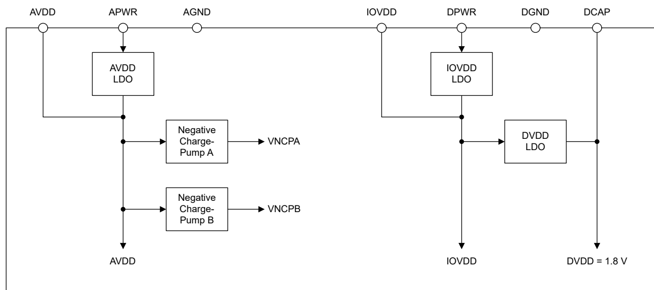
Figure 9-4. Power-Supply Architecture
