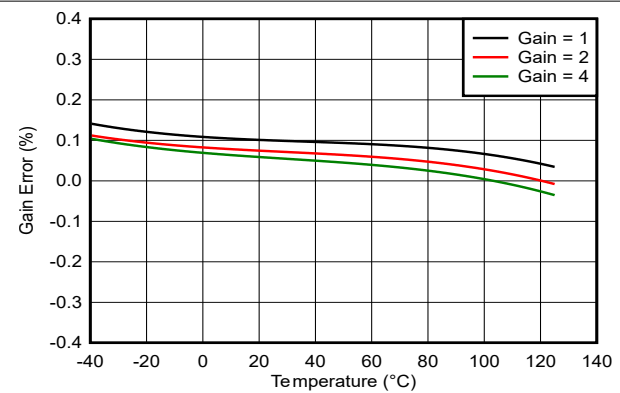
Including error of REFy Figure 5-11. ADC2y Gain Error vs Temperature
