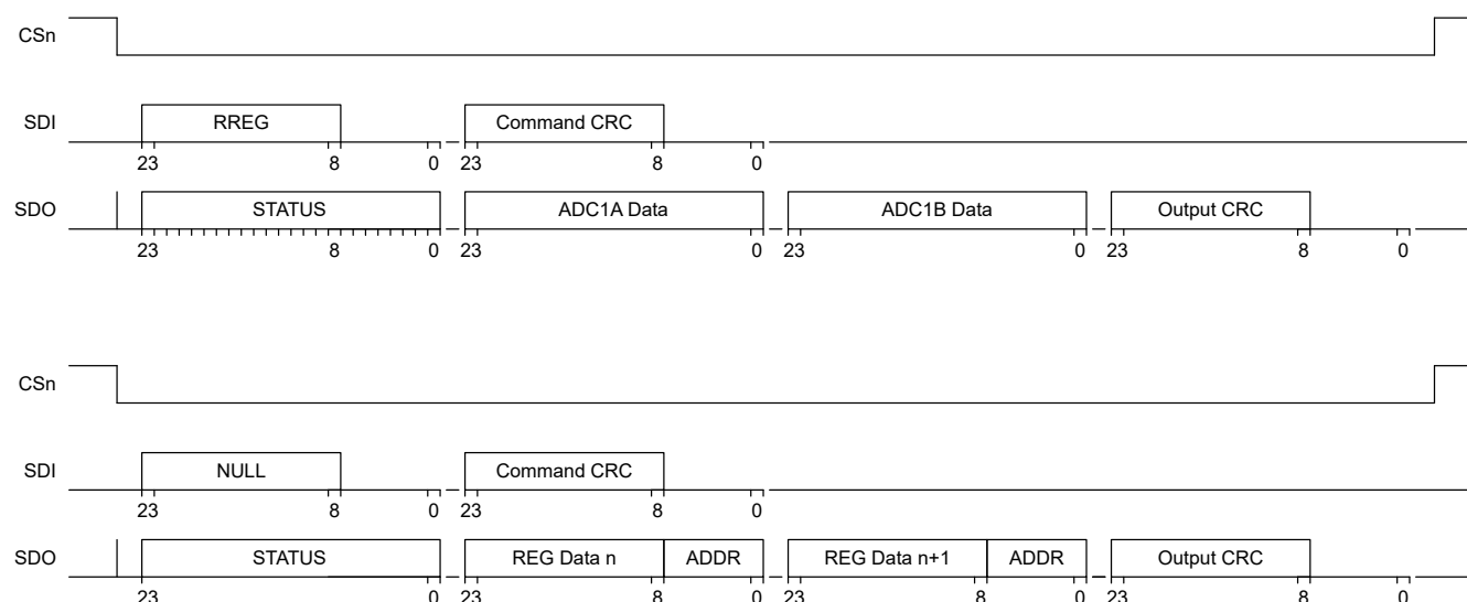
Figure 7-30. Bit Alignment, 24-Bit Word Size, RREG Command
