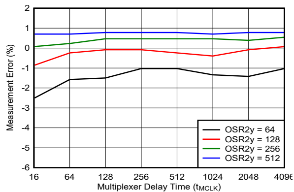
Figure 5-26. ADC2A Supply Voltage Readback Measurement Accuracy
