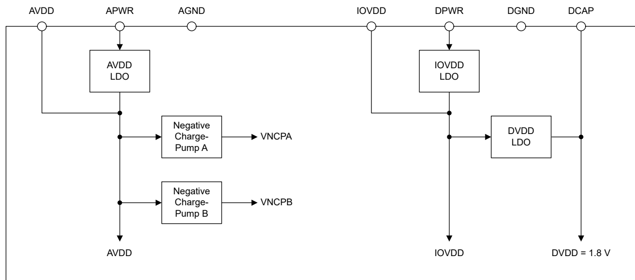
Figure 9-4. Power-Supply Architecture
