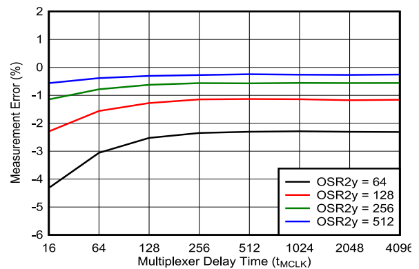
Figure 5-27. ADC2A Supply Voltage Readback Measurement Accuracy
