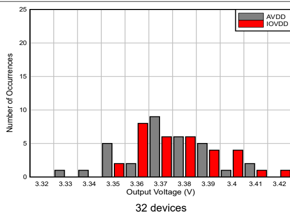
Figure 5-33. AVDD and IOVDD LDO Output Voltage Histogram
