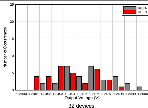
Figure 5-12. REFy Output Voltage Histogram
