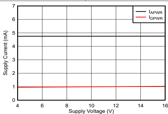
Active mode, all ADCs enabled and converting Figure 5-36. Supply Current vs Supply Voltage
