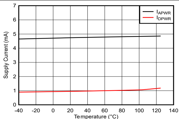
Active mode, all ADCs enabled and converting Figure 5-35. Supply Current vs Temperature
