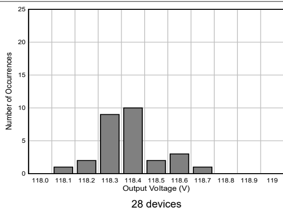
Figure 5-20. Temperature Sensor Output Voltage Histogram
