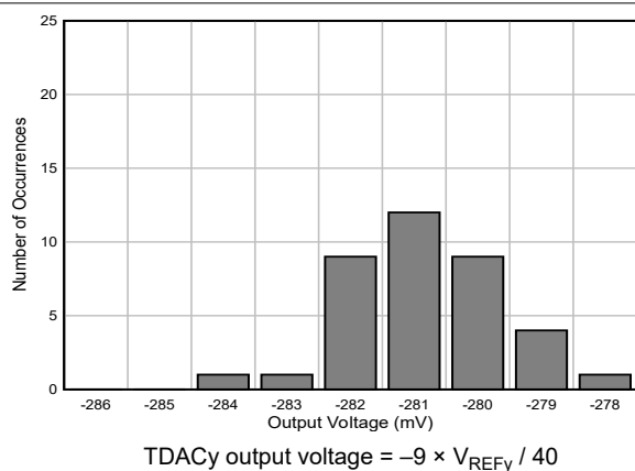
Figure 5-24. Test DACy Output Voltage Histogram
