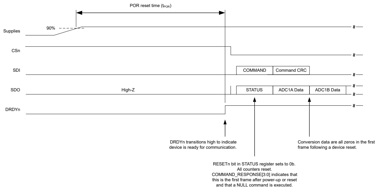
Figure 7-26. DRDYn Pin Behavior After POR
