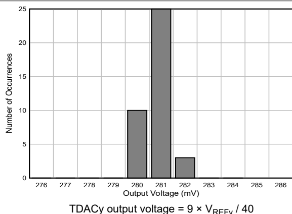
Figure 5-22. Test DACy Output Voltage Histogram
