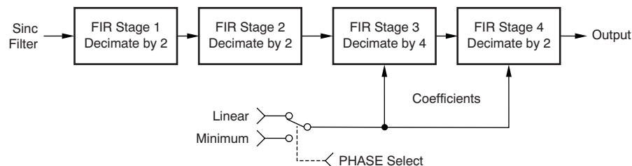
Figure 46. FIR Filter
