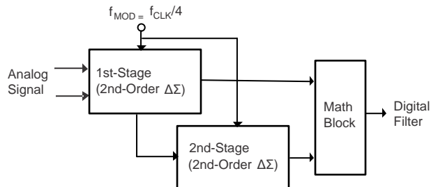
Figure 30. Fourth-Order Modulator
