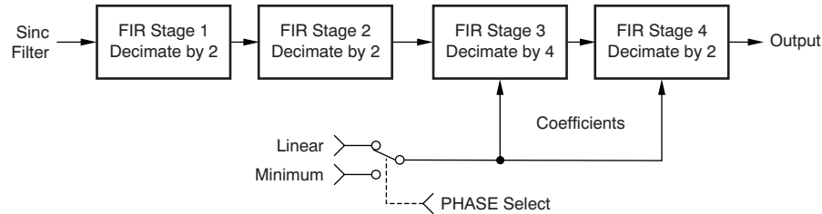
Figure 38. FIR Filter Substages
