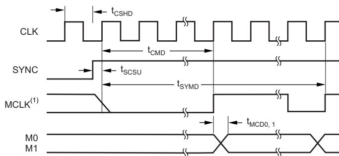
Figure 56. Modulator Mode Timing
