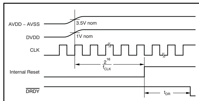
Figure 51. Power-On Sequence
