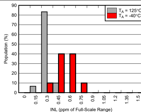
Figure 5-70. INL Distributions
