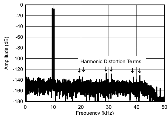
f_1 = 9.7kHz , f_2 = 10.3kHz , V_{IN} = -6.5dBFS Figure 5-62. Intermodulation Distortion FFT
