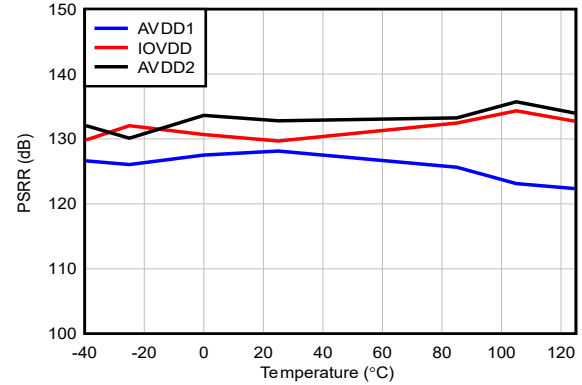
Figure 5-86. DC PSRR vs Temperature
