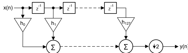
Figure 7-13. FIR3 Filter Structure
