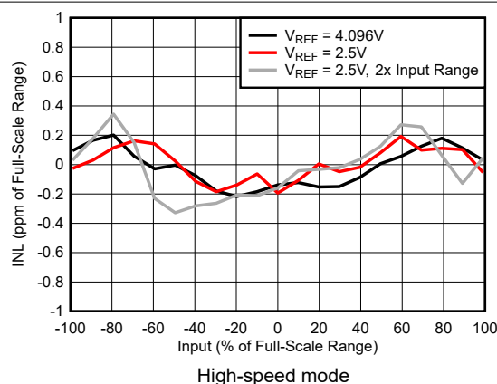
Figure 5-64. INL Error vs Input Voltage
