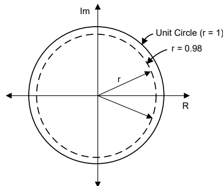
Figure 7-22. Z-Plane
