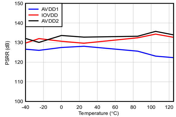
Figure 5-80. DC PSRR vs Temperature
