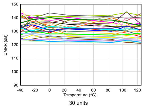
Figure 5-70. DC CMRR vs Temperature
