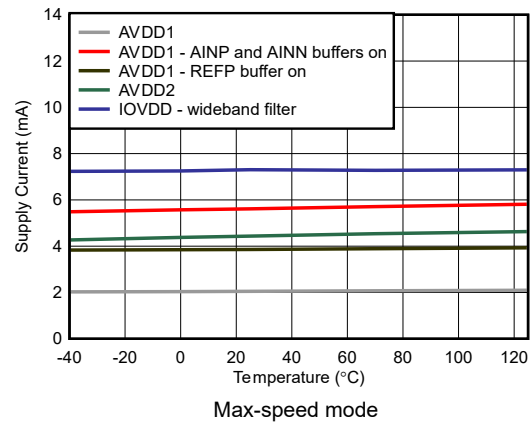
Figure 5-82. Power-Supply Current vs Temperature
