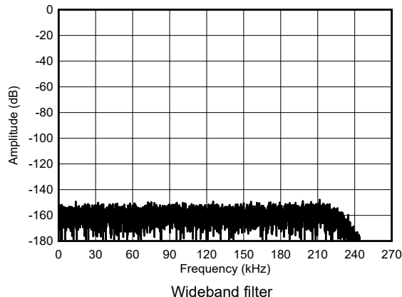
Figure 5-7. Max-Speed Mode, Shorted-Input FFT
