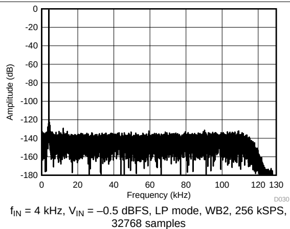
Figure 10. Output Spectrum
