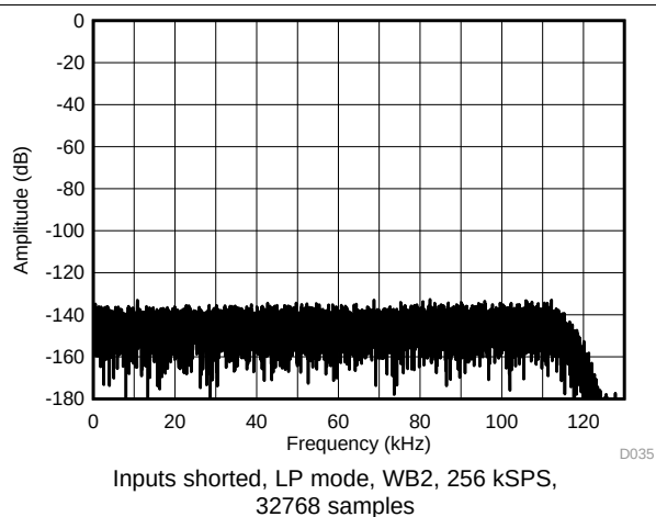
Figure 15. Output Spectrum
