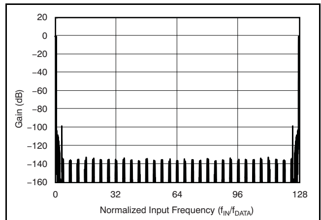
Figure 62. Frequency Response Out to f_{\text{MOD}} for High-Resolution Mode
