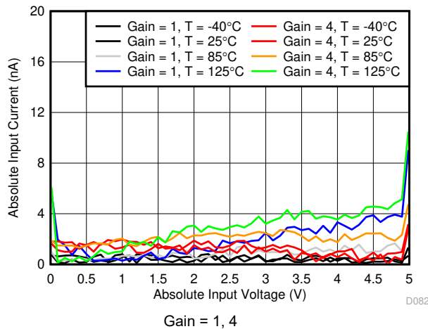
Figure 7-60. ADC2 Absolute Input Current
