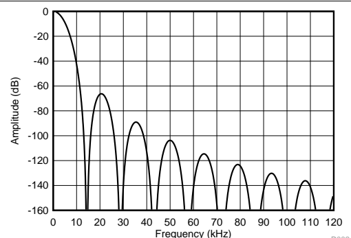
Figure 23. Frequency Response (14400 SPS)
