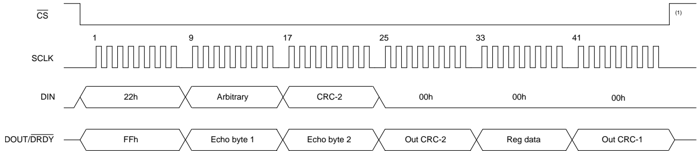
Figure 39. Register Read Operation (address = 02h, CRC Mode Enabled)
