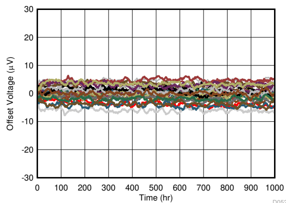
Figure 7-14. Offset Error Drift Distribution
