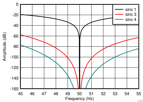
Figure 9-13. Sinc Filter Frequency Response (50 SPS)
