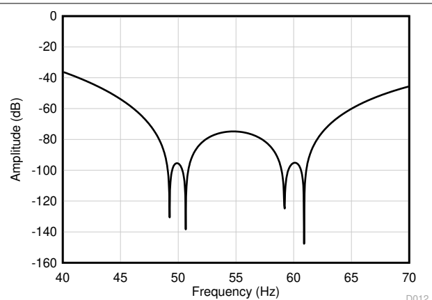
Figure 9-16. FIR Filter Frequency Response Detail (20 SPS)
