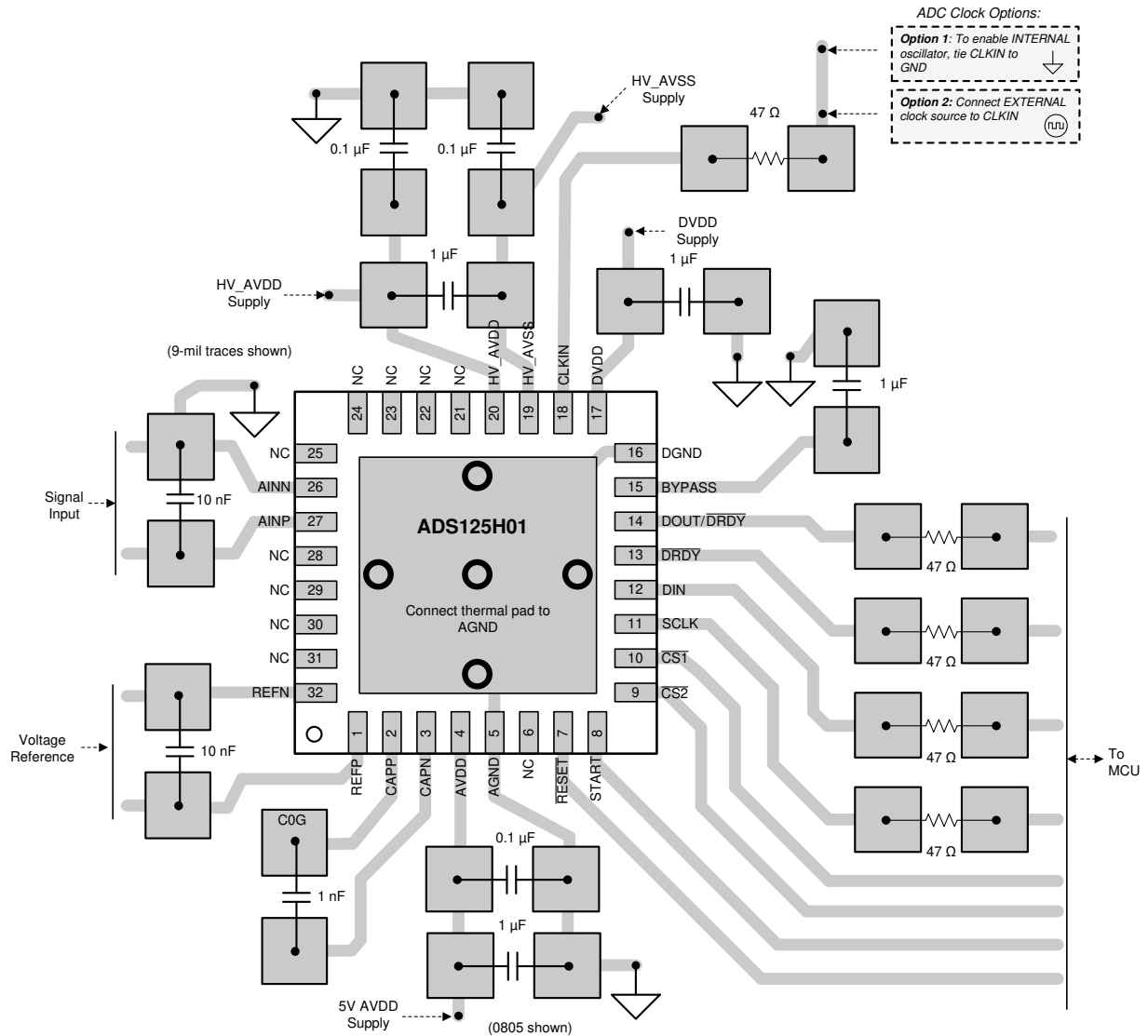
Figure 12-1. Example Top-Layer PCB Layout
