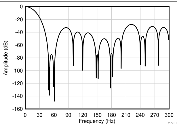
Figure 9-15. FIR Filter Frequency Response (20 SPS)
