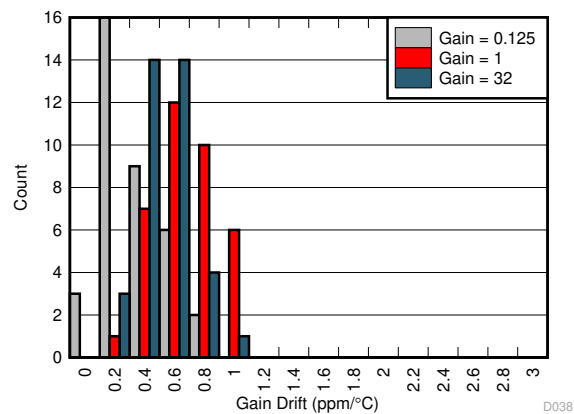
Figure 7-19. Gain Drift Distribution
