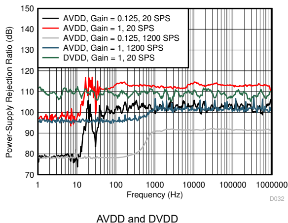
Figure 7-28. PSRR vs Frequency
