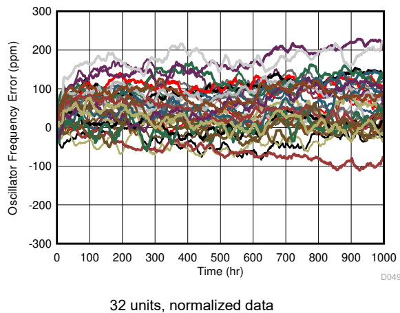
Figure 7-26. Oscillator Frequency Long-Term Drift
