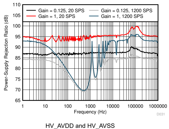
Figure 7-27. PSRR vs Frequency
