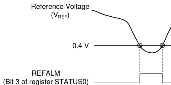
Figure 9-5. Reference Monitor Operation
