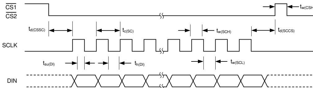
Figure 7-1. Serial Interface Timing Requirements
