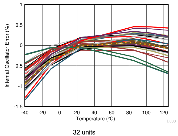
Figure 7-25. Oscillator Frequency Error vs Temperature
