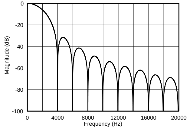
Figure 67. Low-Latency Filter Frequency Response, Data Rate = 2 kSPS
