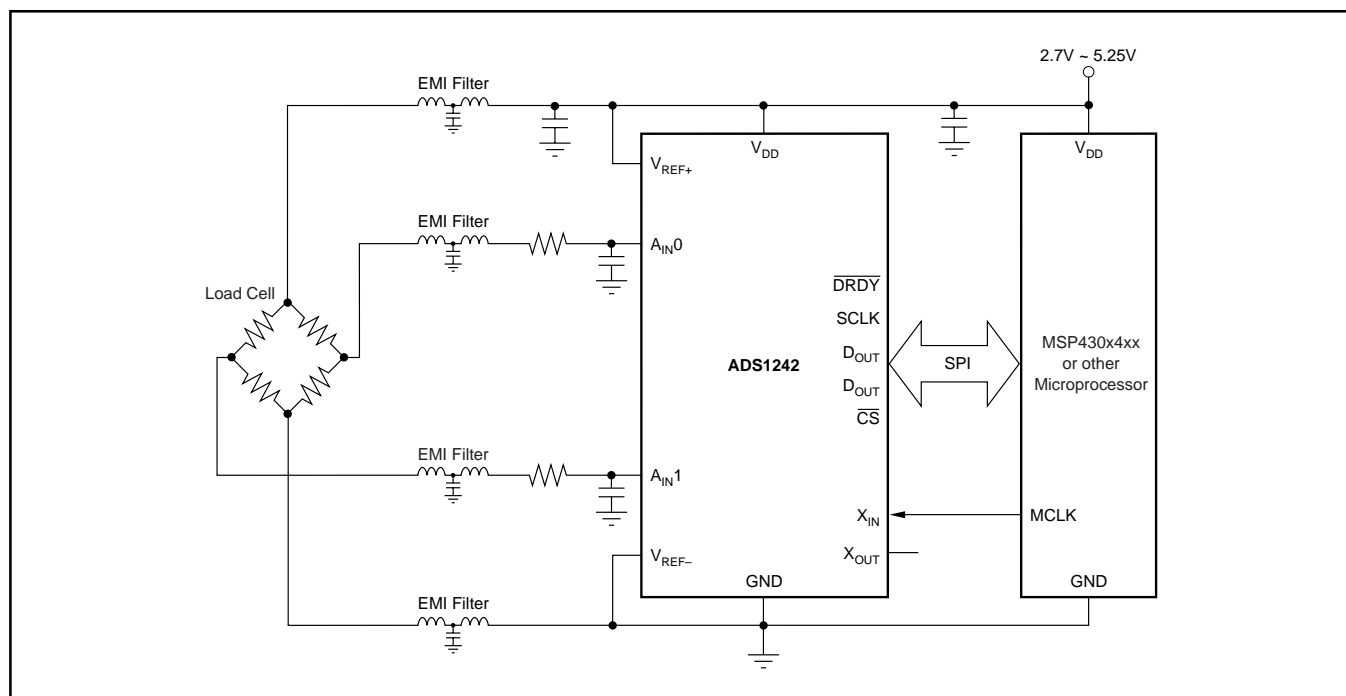
FIGURE 8. Schematic of a General-Purpose Weight Scale.
