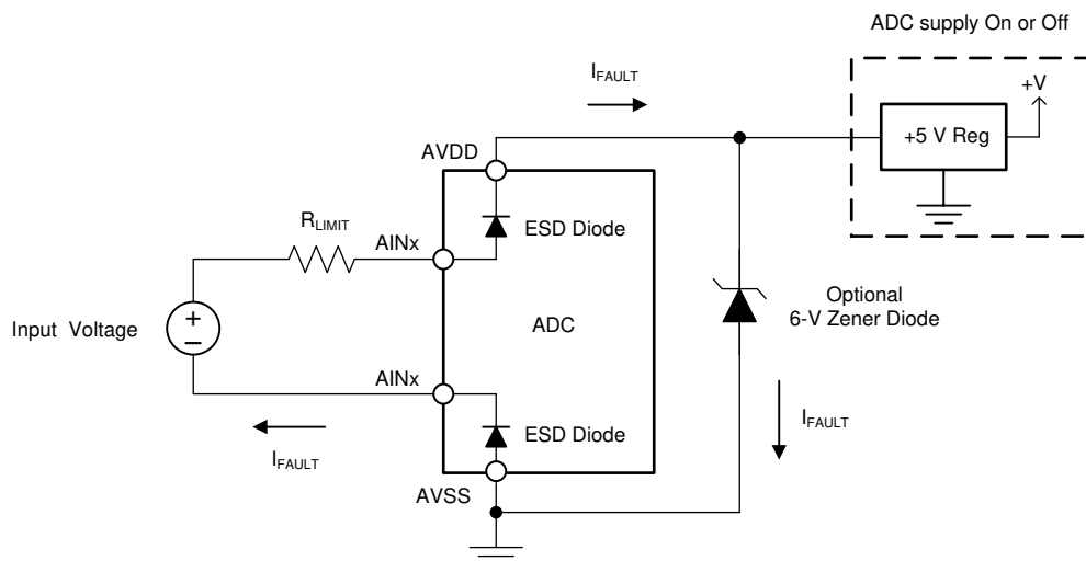
Figure 88. Analog Power-Supply Clamp
