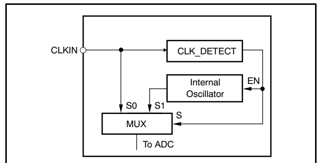
Figure 20. Equivalent Circuitry of the Clock Source
