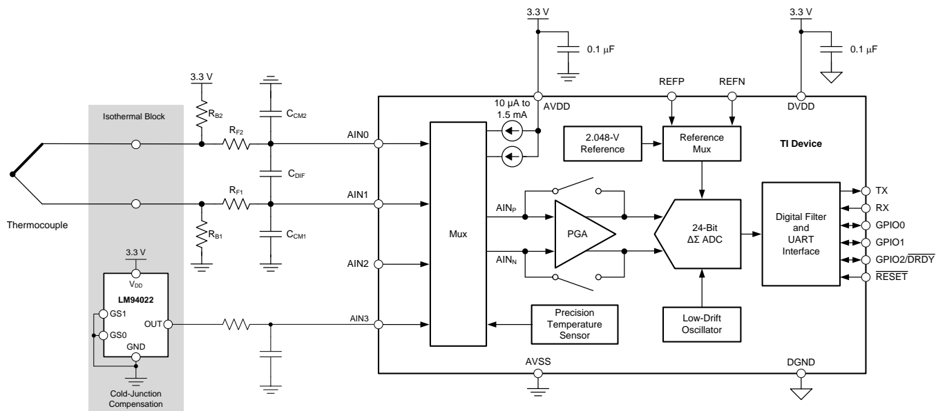
Figure 76. Thermocouple Measurement
