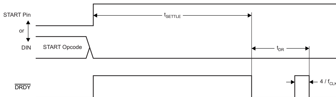
Figure 32. Settling Time
