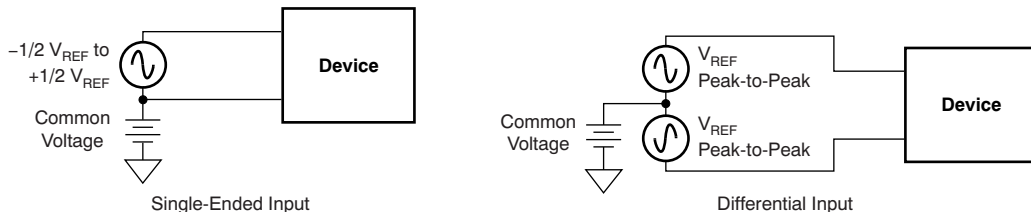
Figure 16. Methods of Driving the ADS1191/2: Single-Ended or Differential
