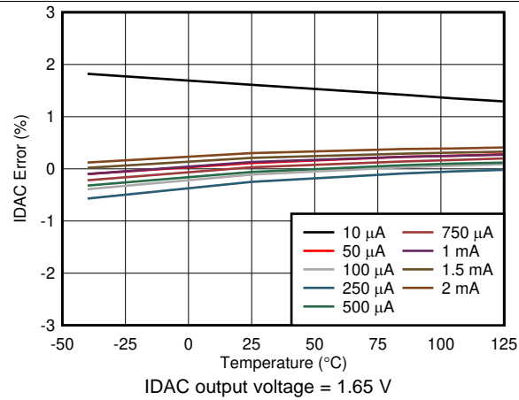
Figure 27. IDAC Accuracy vs Temperature
