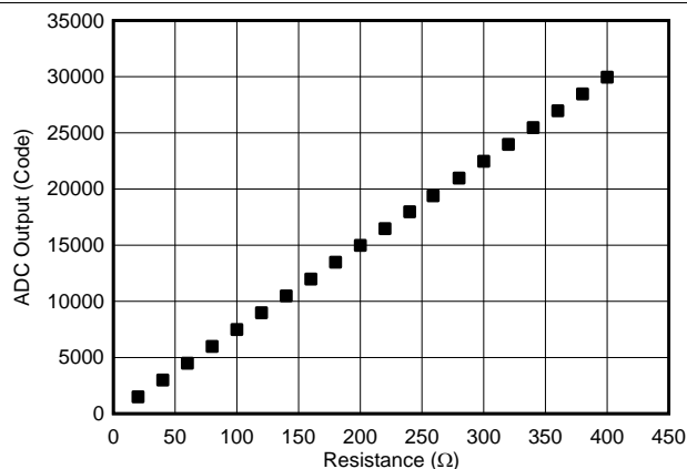
Figure 114. ADC Output Code vs Equivalent RTD Resistance
