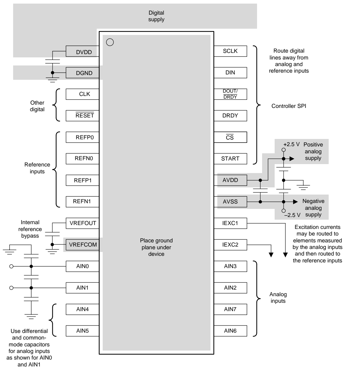
Figure 79. Layout Example
