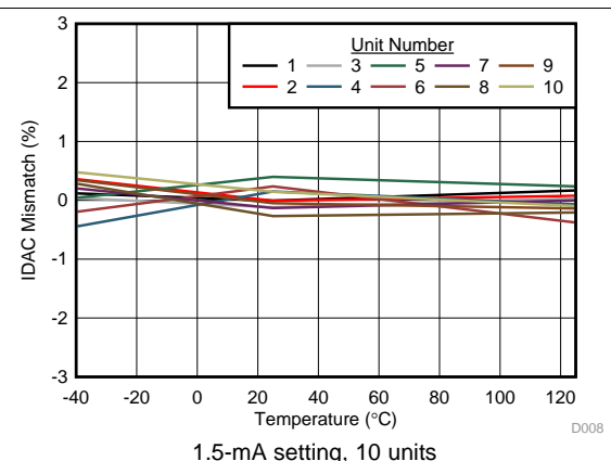
Figure 8. IDAC Drift
