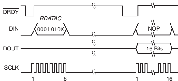
Figure 49. RDATA: Read Data Continuously Command
