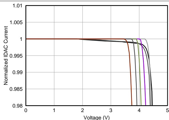
Figure 8. IDAC Drift
