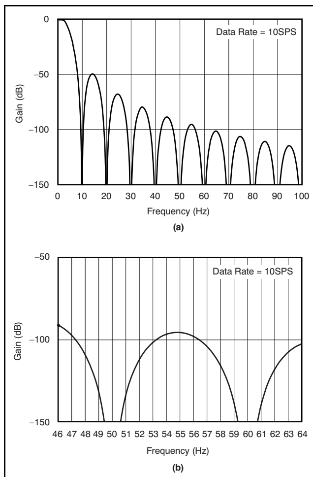
Figure 4. Frequency Response Out To 100Hz
