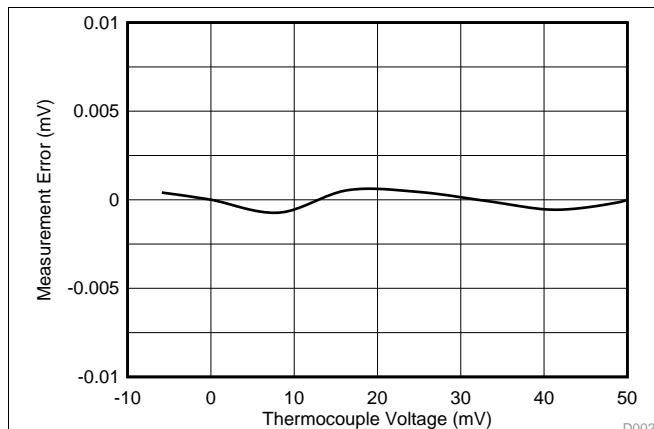
Figure 77. Voltage Measurement Error vs V_{\text{TC}}
